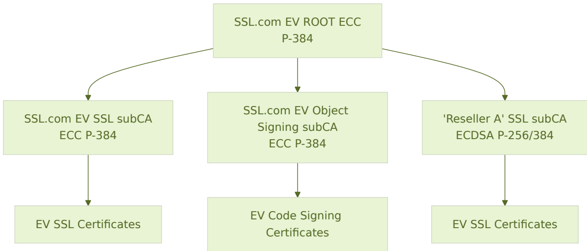
Figure 4: SSL.com Original EV ECC CA Hierarchy
